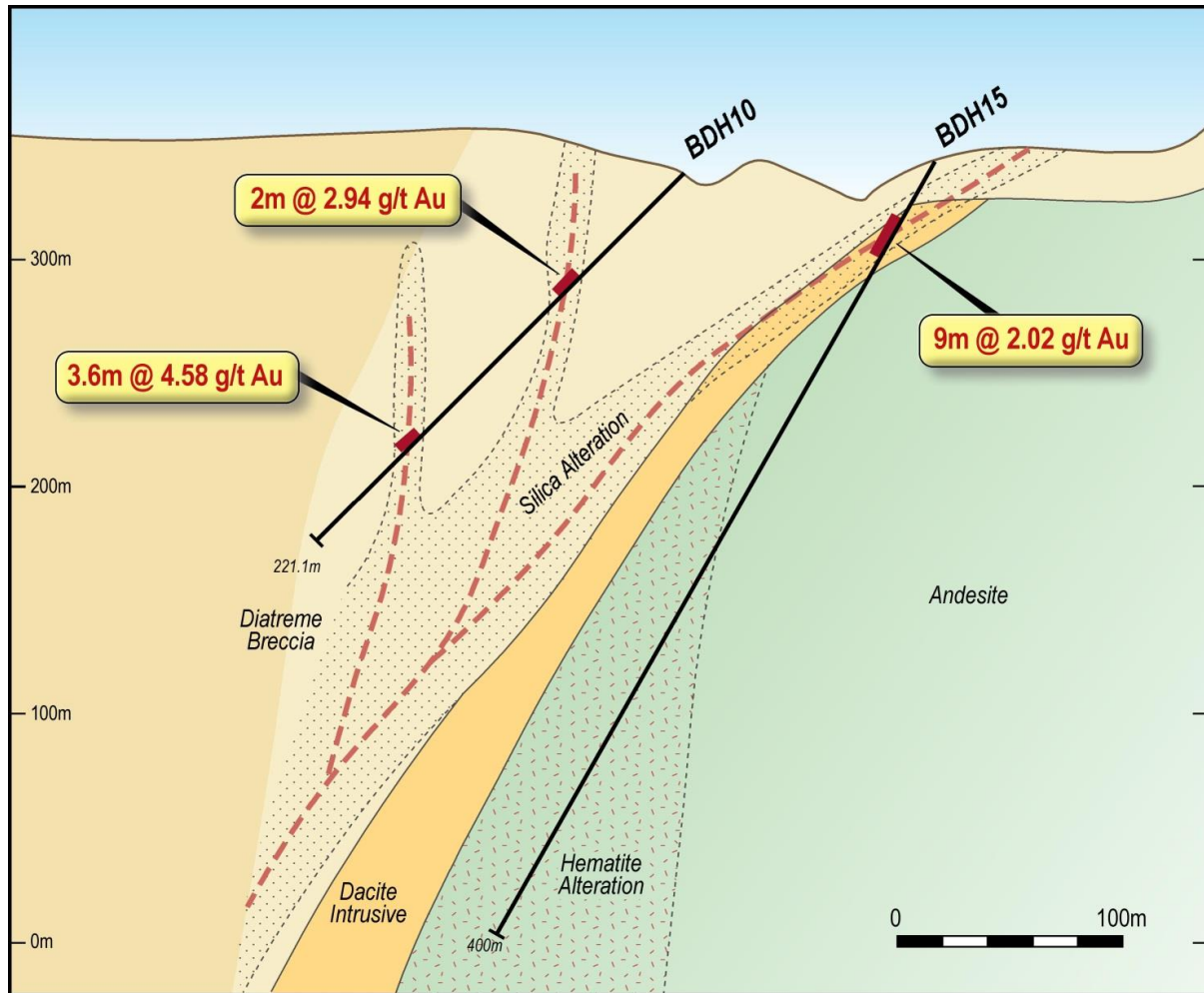
Figure 5 – Bunawan BDH15 & BDH10 interpretive geological cross-section showing mineralisation on the edge of the diatreme and the newly found mineralised Dacite.
